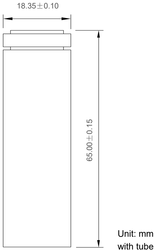
Fig. 1. Outline Dimensions of INR18650/29gge
